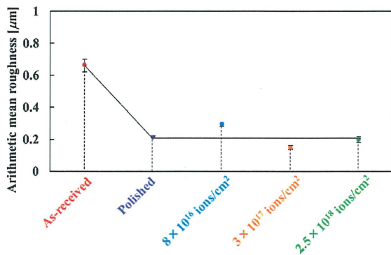
Fig. 11 Arithmetic mean surface roughness for five kinds of materials
