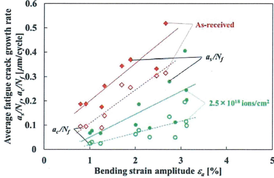
Fig. 9 Dependence of average fatigue crack growth rates a_s/N_f and a_o/N_f on bending strain amplitude \varepsilon_a for tapes as-received and ion-implanted with 2.5 \times 10^{18} ions/cm 2 : a_s/N_f is shown by closed symbols and a_o/N_f by open symbols
