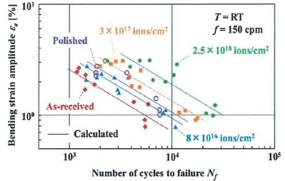
Fig. 2 Relationship between bending strain amplitude and the number of cycles to failure.
