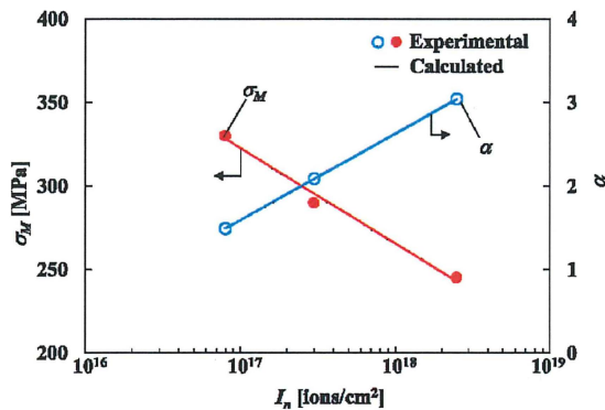
Fig. 12 Dependence of \sigma_M and \alpha on I_n
