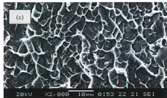
Fig. 5 SEM photograph of the typical fracture surface of polished tape for \varepsilon_a = 2.42\% and N_f = 3615
