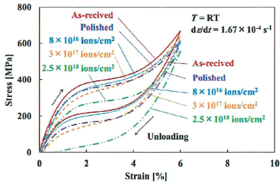
Fig. 1 Stress-strain curves
