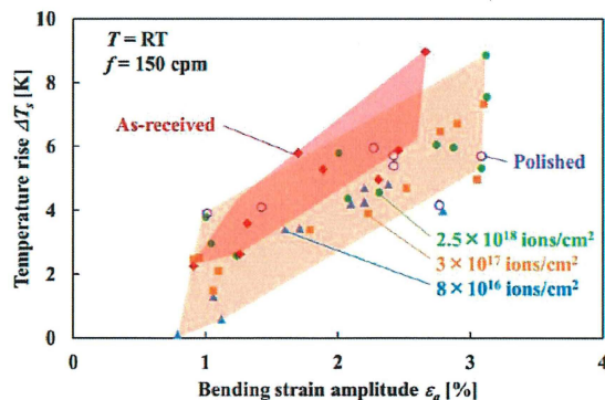
Fig. 3 Relationship between saturated temperature rise \Delta T_s and bending strain amplitude \varepsilon_a .
