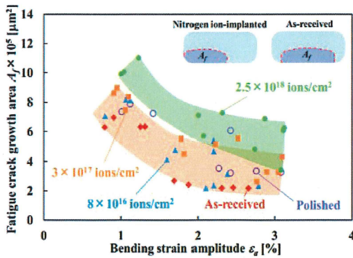
Fig. 7 Relationship between fatigue crack growth area and bending strain amplitude
