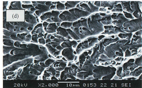
Fig. 6 SEM photographs of the typical fracture surface of ion-implanted tape with 2.5 \times 10^{18} ions/cm 2 for \varepsilon_a = 3.12\% and N_f = 6018 : (a) whole fracture surface, (b) crack initiation part (1), (c) central fracture part (2), and (d) final fracture part (3)
