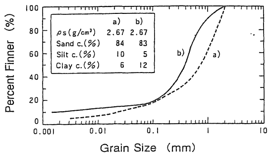
Fig.3.5 Grain Size Distribution of Fill Materials used in Tests
