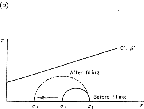
Fig.3.1 Stress Change due to Differential Settlement
