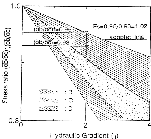
Fig.4.3 Safety Evaluation with Stress Ratio
