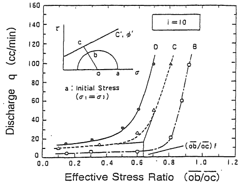
Fig.3.7 Discharge versus Stress Ratio Relation (Test-1)
