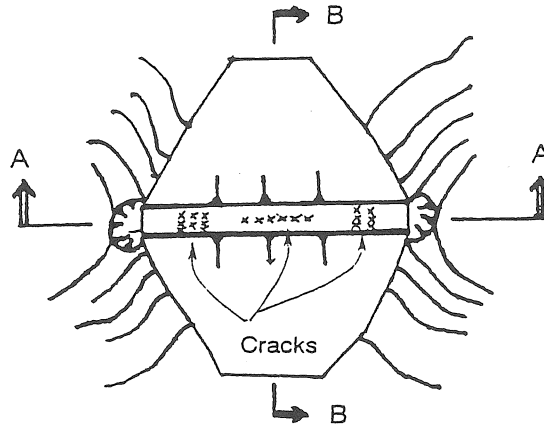
(a) Plan View of Rock Fill Dam
