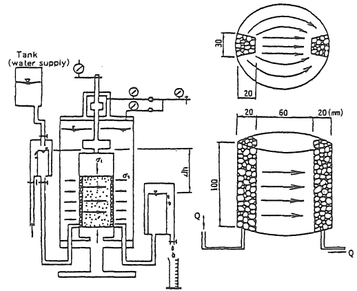
Fig.3.3 Seepage Test Apparatus for Test-1 Series
