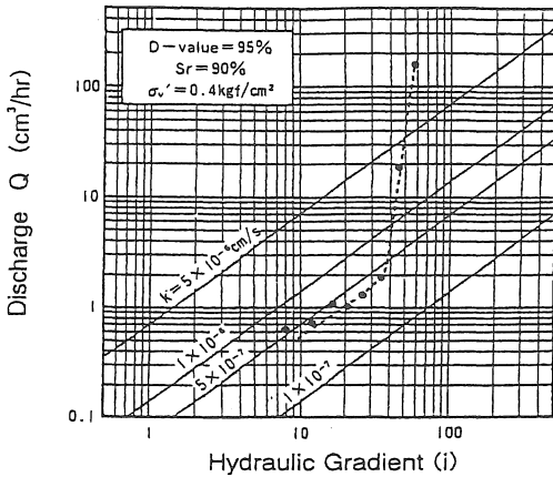
Fig.3.9 Discharge versus Hydraulic Gradient Relation (Test-2)
