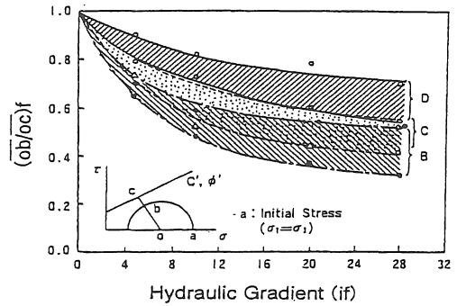
Fig.3.8 Stress Ratio at Failure (Test-1)
