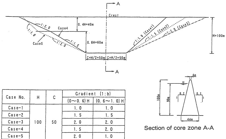
Fig.4.1 Abutment Configuration Employed in Dynamic Response Analysis
