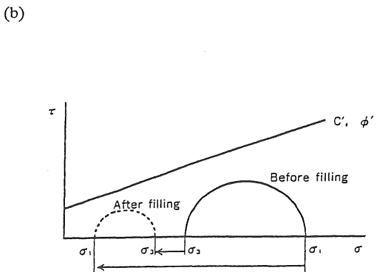
Fig.3.2 Stress Change due to Arch Action
