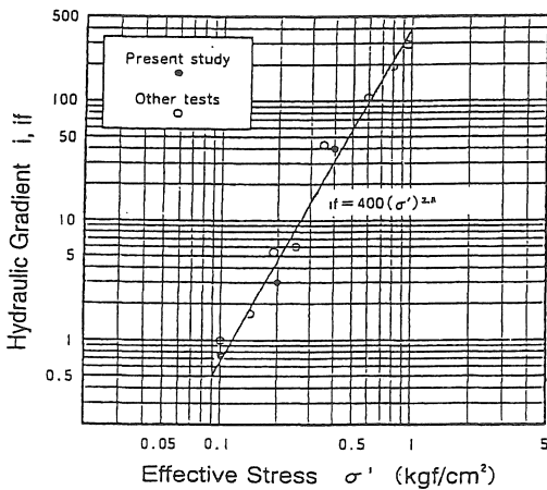
Fig.3.10 Hydraulic Gradient at Failure (Test-2)
