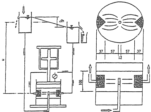
Fig.3.4 Seepage Test Apparatus for Test-2 Series
