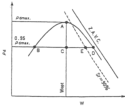
Fig.3.6 Compaction Conditions of Test Specimens
