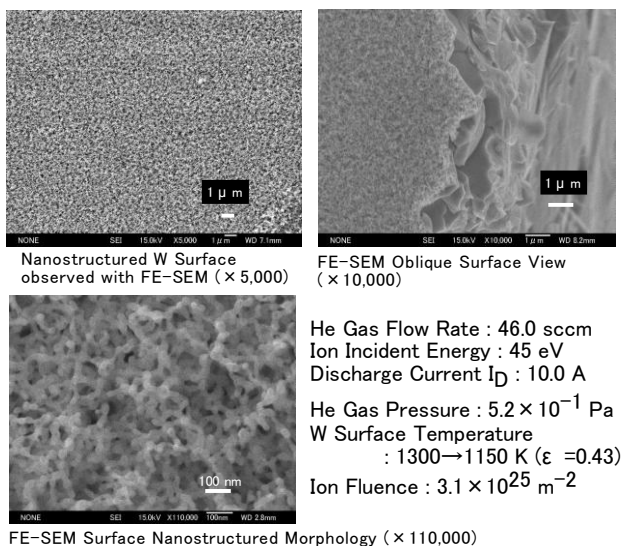
Fig.11 FE-SEM photos of arborescent nanostructure on the tungsten surface at around 1000 °C.
