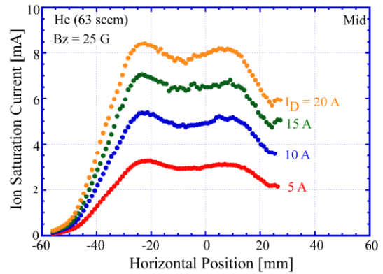
Fig.5 Horizontal profiles of ion saturation current, taking the discharge current I_D as a parameter.
