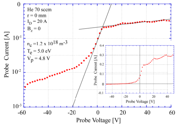
Fig.6 Logarithmic plot of electron current collected with a single Langmuir probe as a function of applied voltage with respect to the grounded chamber.
