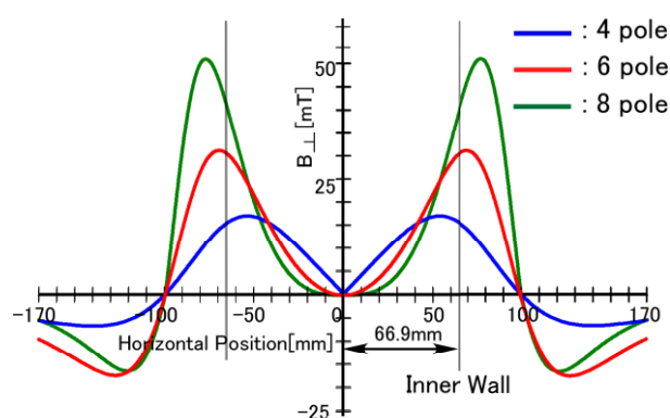
Fig.3 Horizontal distributions of vertical magnetic field for different kinds of multi-cusp configurations.
