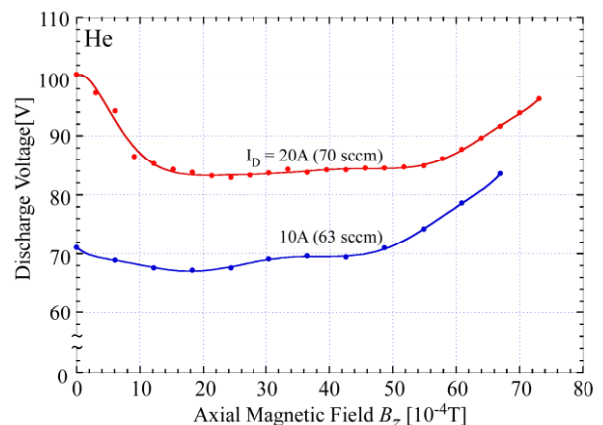
Fig.10 Dependence of the discharge voltage on the axial magnetic field for two different fixed discharge current I_D = 10 and 20 A.
