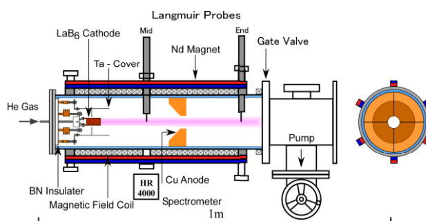
Fig.1 Schematic view of the device AIT-PID
