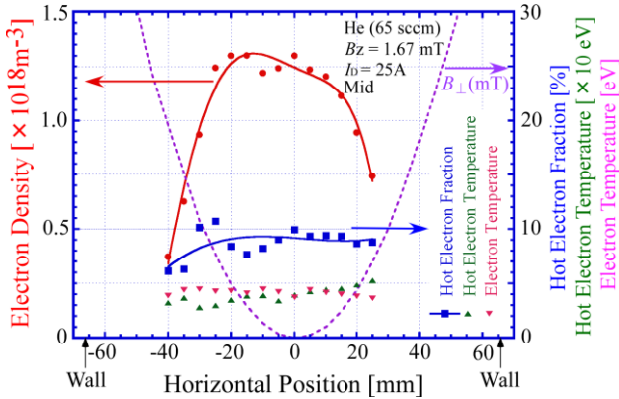
Fig.7 Horizontal profiles of electron density, bulk and hot electron temperatures and hot electron fraction at the discharge current I_D of 25 A.
