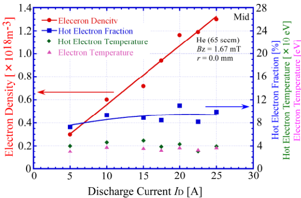
Fig.8 Dependence of the plasma parameters on the discharge current.
