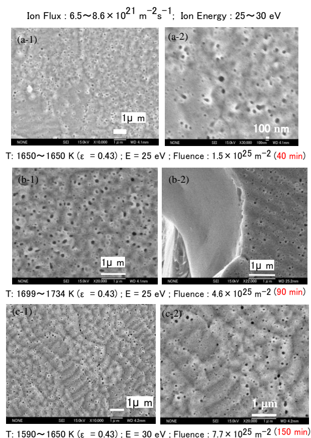
Fig.12 FE-SEM photos of small bubbles and holes on the tungsten surface at high surface temperature.
