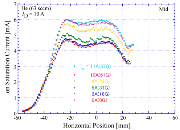
Fig.9 Horizontal profiles of ion saturation current, taking the intensity of axial magnetic field as a parameter.
