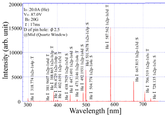
Fig.4 Light emission spectrum from He discharge plasma from ultraviolet through near-infrared lines.
